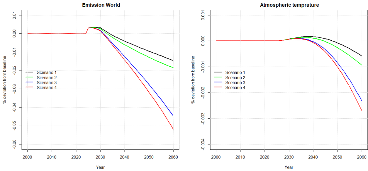
Figure 5-18 Change in world emission and atmospheric temprature
