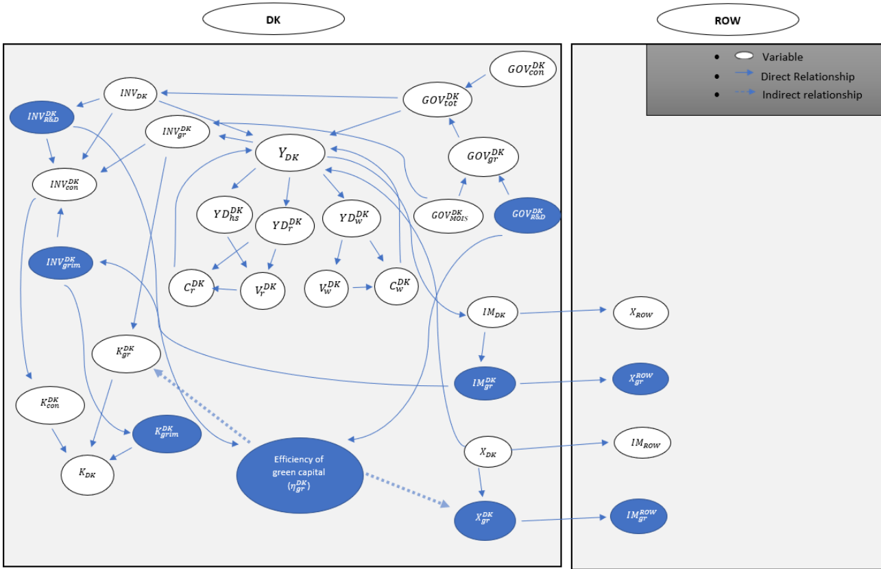
Figure 4-1 DAG presenting the Danish economy and the relations to ROW
